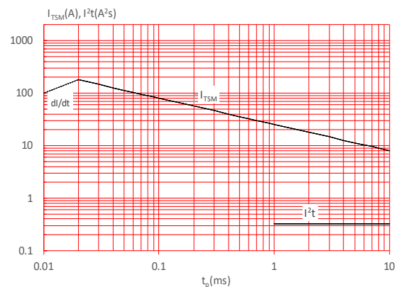
FIG.6: Non-repetitive surge peak on-state current for a sinusoidal pulse with width t_p < 10ms , and corresponding value of I^2t ( dI/dt < 50A/\mu s )
