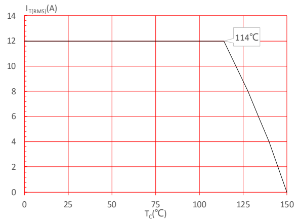
FIG.4: On-state characteristic
